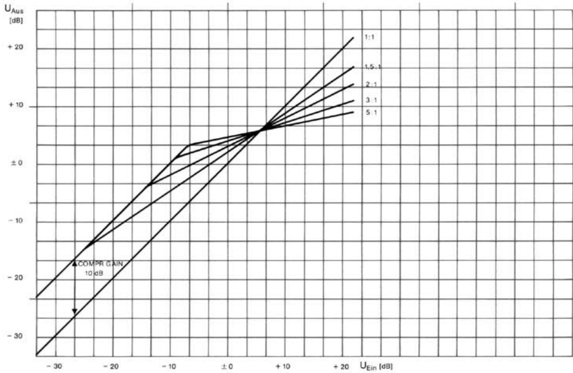
Compressorkennlinie Expander: aus, Output gain: 0 dB
